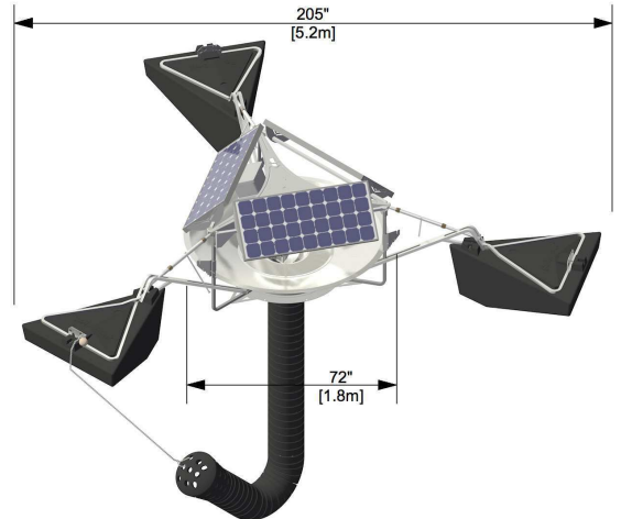
Figure 1: SB2500
