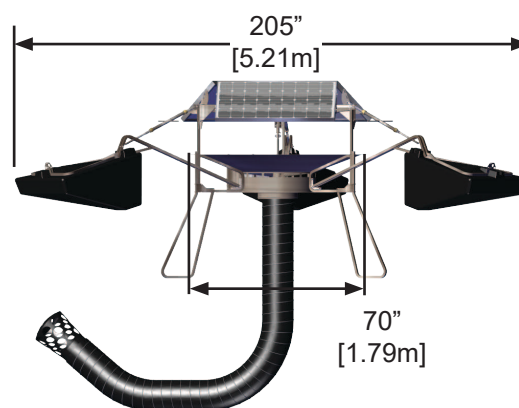
Figure 1: SB10000DM
