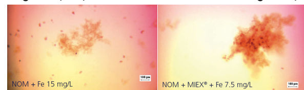
Figure 1: Example of flocs formed from Albert Raw Water with: 15mg/L Fe (left), MIEX® Pretreatment and 7.5mg/L Fe (right)
