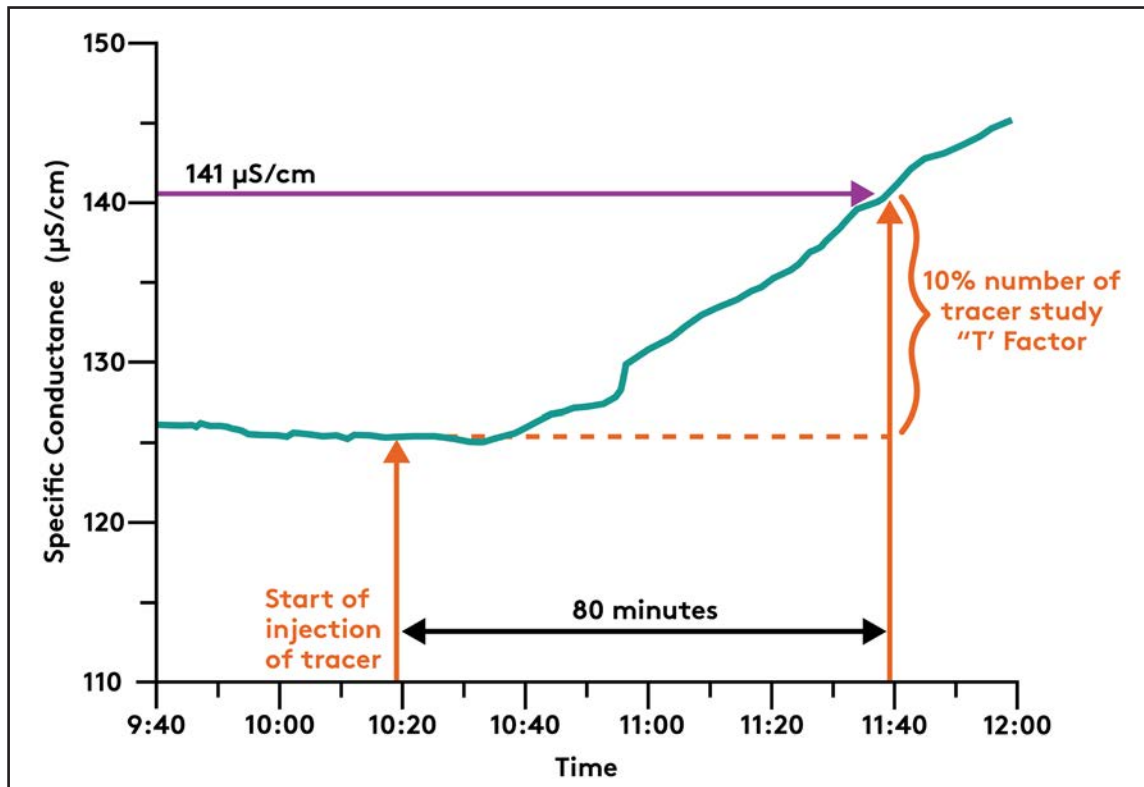
Figure 1 – Tracer Study Results
