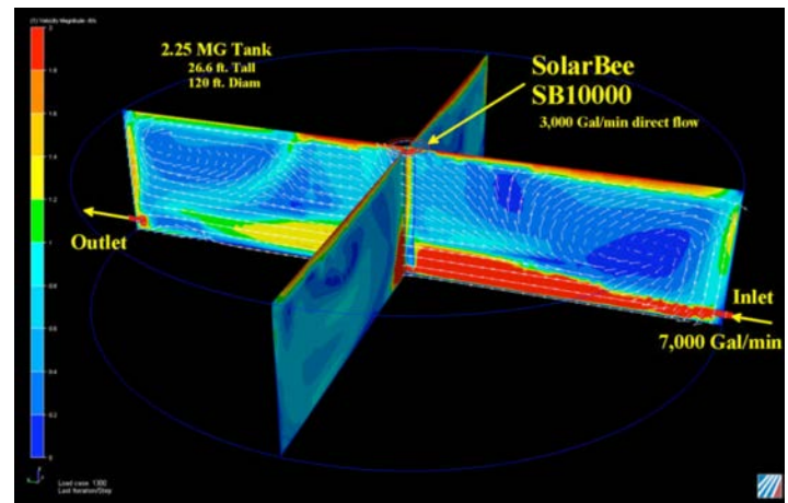
Figure 3–Active mixing with SolarBee®
